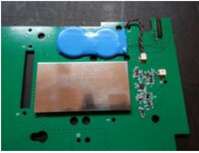
Modified version of the phone largest circuit board (with surveillance device). The battery pack (in blue) and the shielded module (in light brown) are part of the surveillance device.
