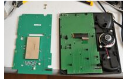
On the left: modified version of the phone largest circuit board (with surveillance device) without the battery pack. On the right: unmodified version.
